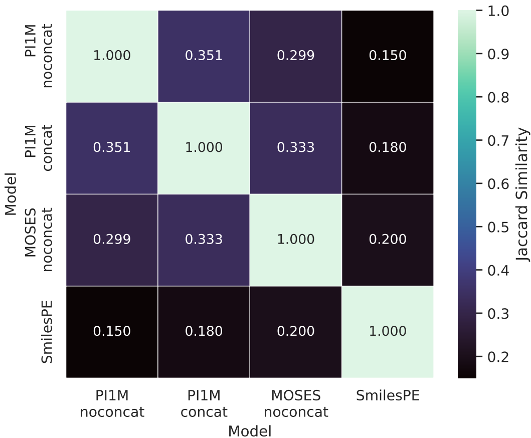
Token Vocabulary Overlap Between Models
