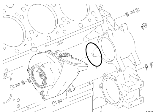
COOLANT PUMP HIGH-TEMP CIRCUIT XS524200.00004
