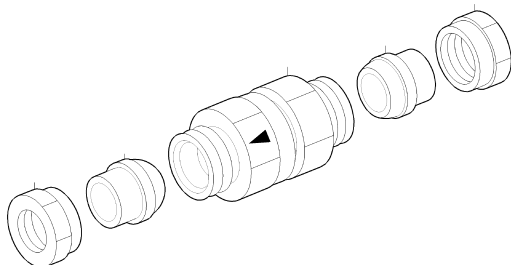
NON-RETURN VALVE FOR OIL PRIMING PUM 180.00443
