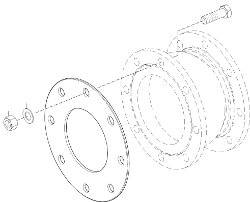
CONNECTION PARTS FOR SEAWATER XS527200.00062
