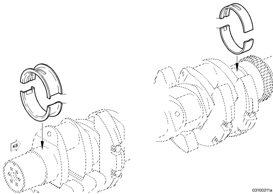
MAIN BEARING 030.00656
