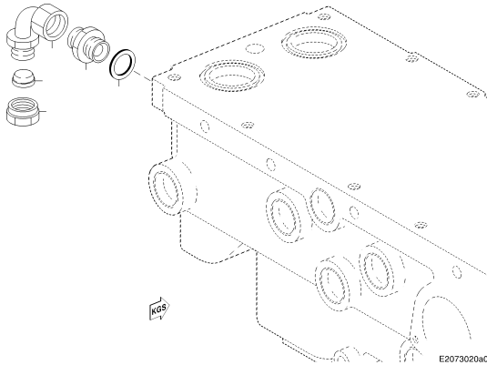
CONNECTING HARDWARE FOR PREHEATING UNIT 200.00030
