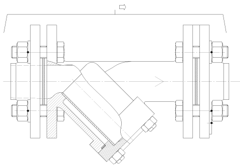
DIRT TRAP FOR FUEL X00039280
