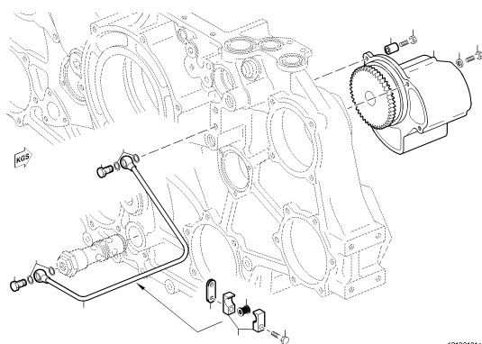
OIL SYSTEM BASIC SCOPE X00010483
