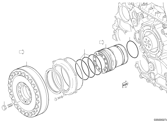
VIBRATION DAMPER 030.00485
