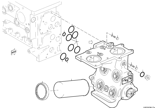
OIL FILTER X00021913
