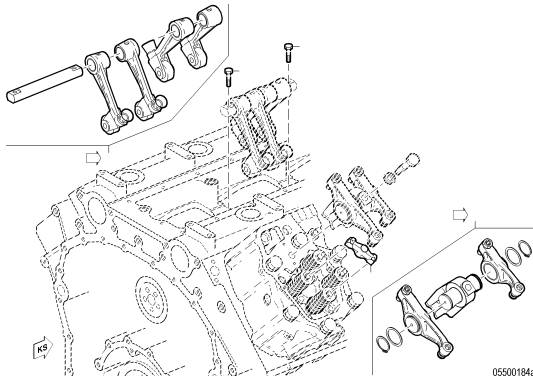
VALVE GEAR 050.00065
