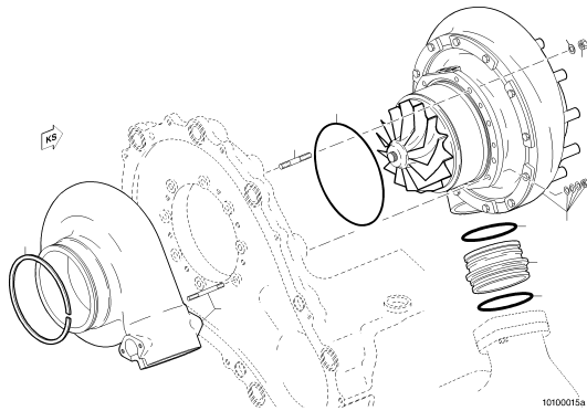
EXHAUST TURBOCHARGER LEFT X00039533
