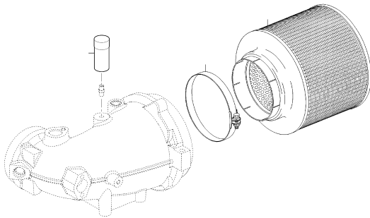
AIR FILTER 120.00007
