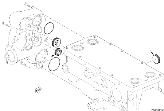
RESTRICTOR 200.00547
