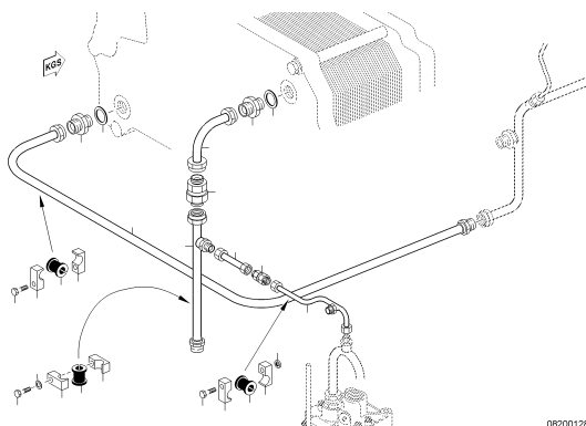
SEAWATER COOLER X00030235
