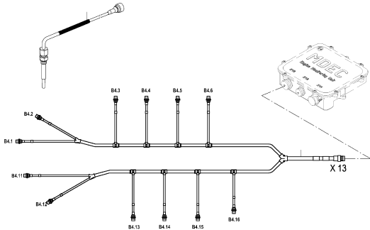
ENGINE CABLING ON ENGINE 500.00280
