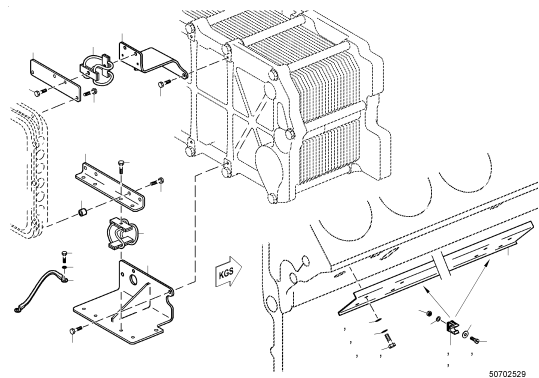
RETAINER F. WIRING HARNESS XS526500.00023
