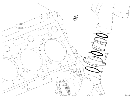
COOLANT DUCTING 200.00605
