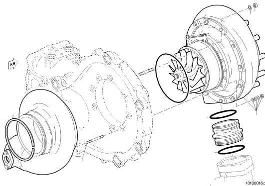
EXHAUST TURBOCHARGER RIGHT X00039534
