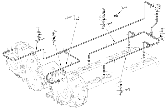
COOLANT VENT 200.00600
