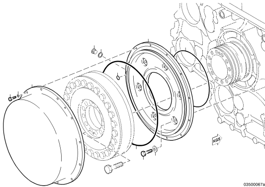
VIBRATION DAMPER HSG 030.00387
