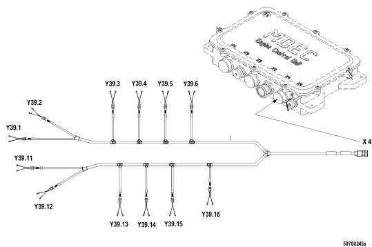
ENGINE CABLING 500.00987
