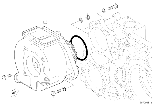
SEAWATER PUMP XS526200.00009
