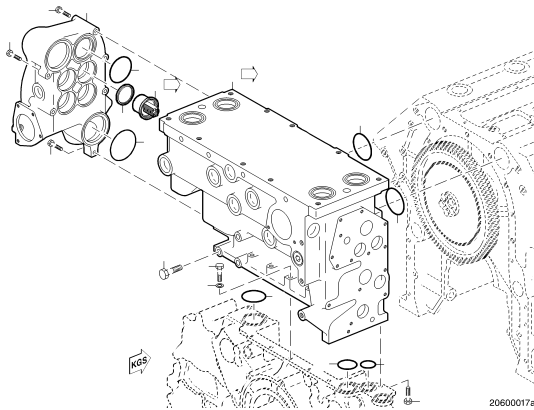
COOLANT DISTRIB HSG W/ATTACHING HARDWAR 200.00120
