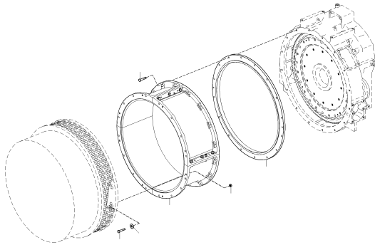
BELL HOUSING FOR ALTERNATOR X00029665
