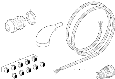
CABLING FOR ON-BOARD GENSET XK00E500.746010-15
