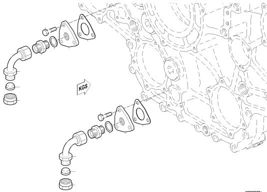
CONNECTIONS FOR OIL PRIMING PPS 180.00038
