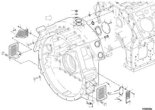
FLYWHEEL HOUSING 010.00365
