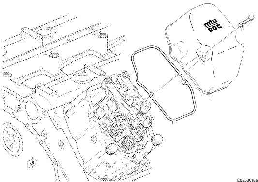
CYLINDER HEAD COVER 050.00094
