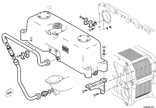
EXPANSION TANK 200.00540
