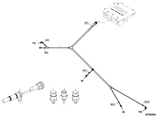
ENGINE CABLING ON ENGINE 500.00274
