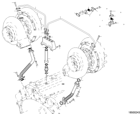
T/CHARGER OIL SUPPLY 180.00459
