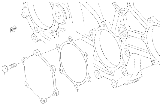
COVER 020.00004
