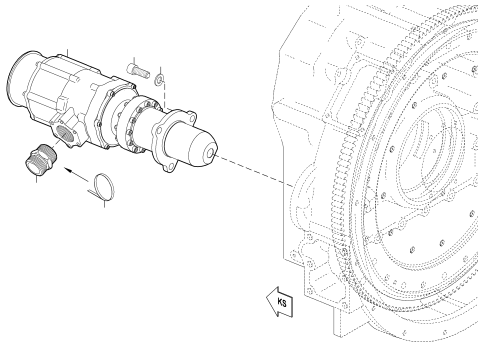
05 STARTER FOR COMPRESSED AIR 170.00142
