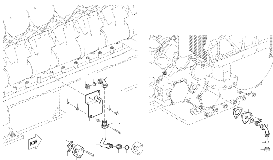
15 CONNECTIONS XS596180.00049
