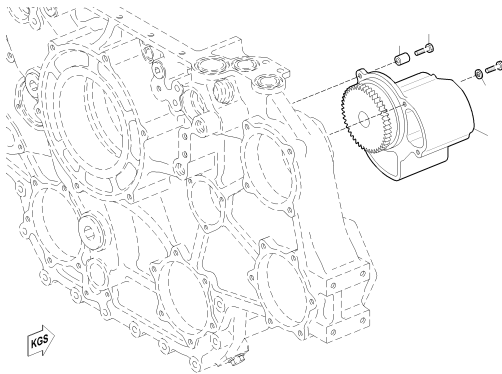
05 OIL PUMP XS528180.00011
