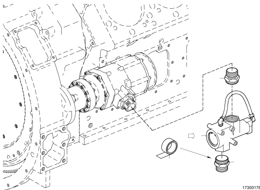
10 CONNECTING HARDWARE FOR AIR START 170.00143
