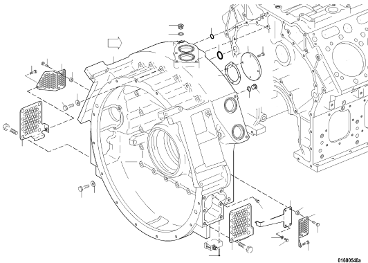
FLYWHEEL HOUSING 010.00365
