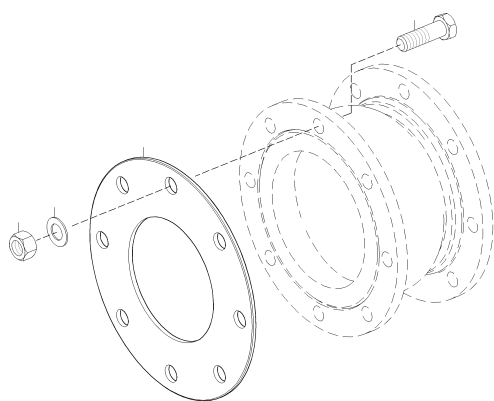
CONNECTION PARTS FOR SEAWATER XS527200.00062
