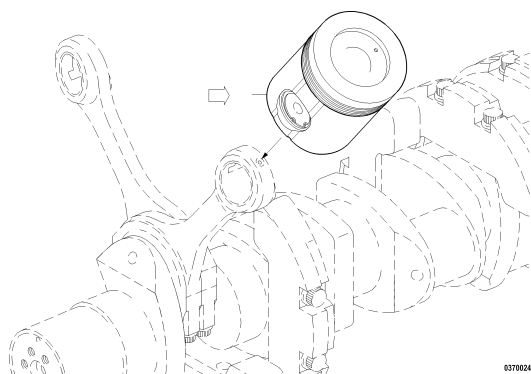
PISTON X00009734
