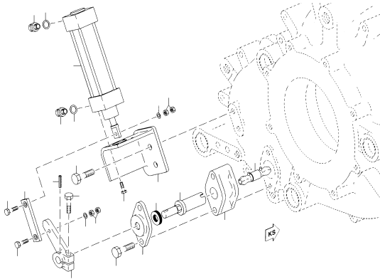
EXHAUST FLAP W/CONTROL 140.00235
