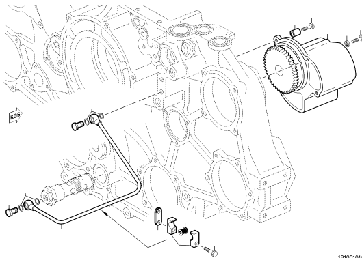
OIL SYSTEM BASIC SCOPE X00010483
