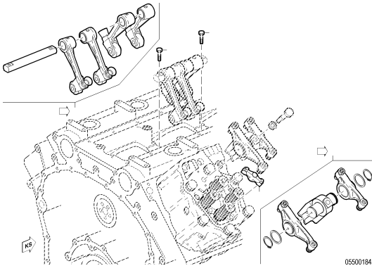
VALVE GEAR 050.00065
