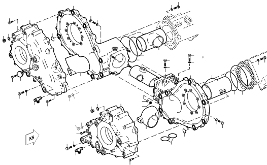
CARRIER HOUSING 140.00233
