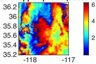
observed wrapped phase (descending)
