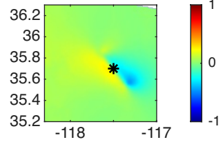
differenced LOS displacement (m) RMS = 0.1002 m
