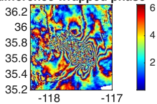
difference wrapped phase
