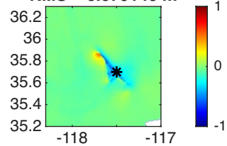
differenced LOS displacement (m) RMS = 0.079146 m
