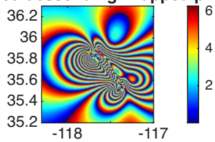
modeled descending wrapped phase
