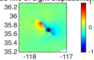
observed line of sight displacement (m)
