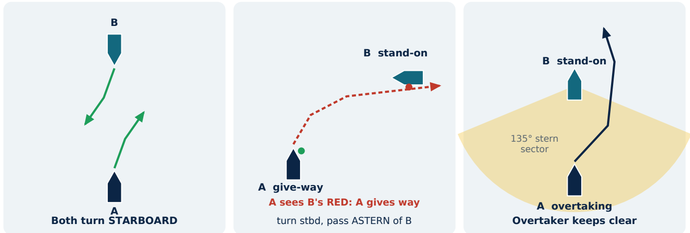
Left to right: Head-on (Rule 14) · Crossing (Rule 15) · Overtaking (Rule 13)
