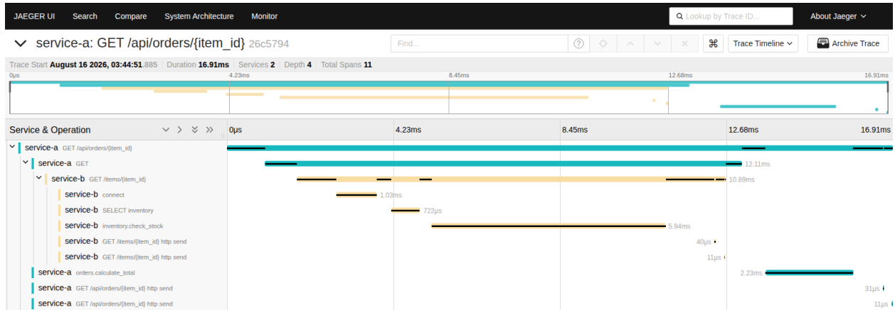
Fig. 2 — Jaeger UI: traza end-to-end service-a → service-b → PostgreSQL con spans custom (trace_id 26c5794...).
