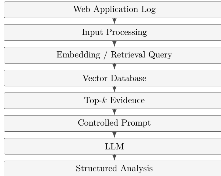
Figure 2.2: Conceptual RAG workflow for web application log analysis.
