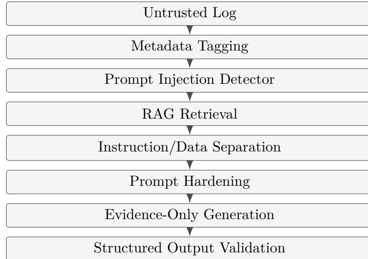
Figure 2.5: Defense-in-depth flow for the defended RAG configuration.
