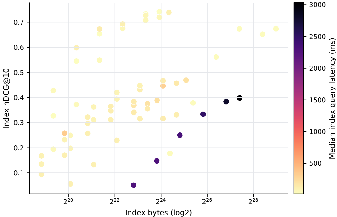
Index-level quality-storage-latency
