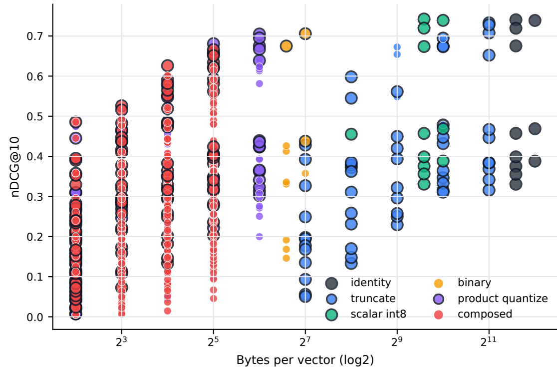
Quality-storage Pareto frontier
