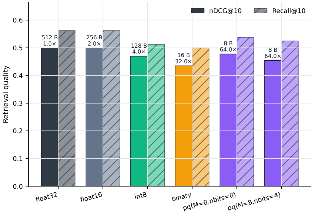
Storage-mode comparison: quality vs. bytes per vector
