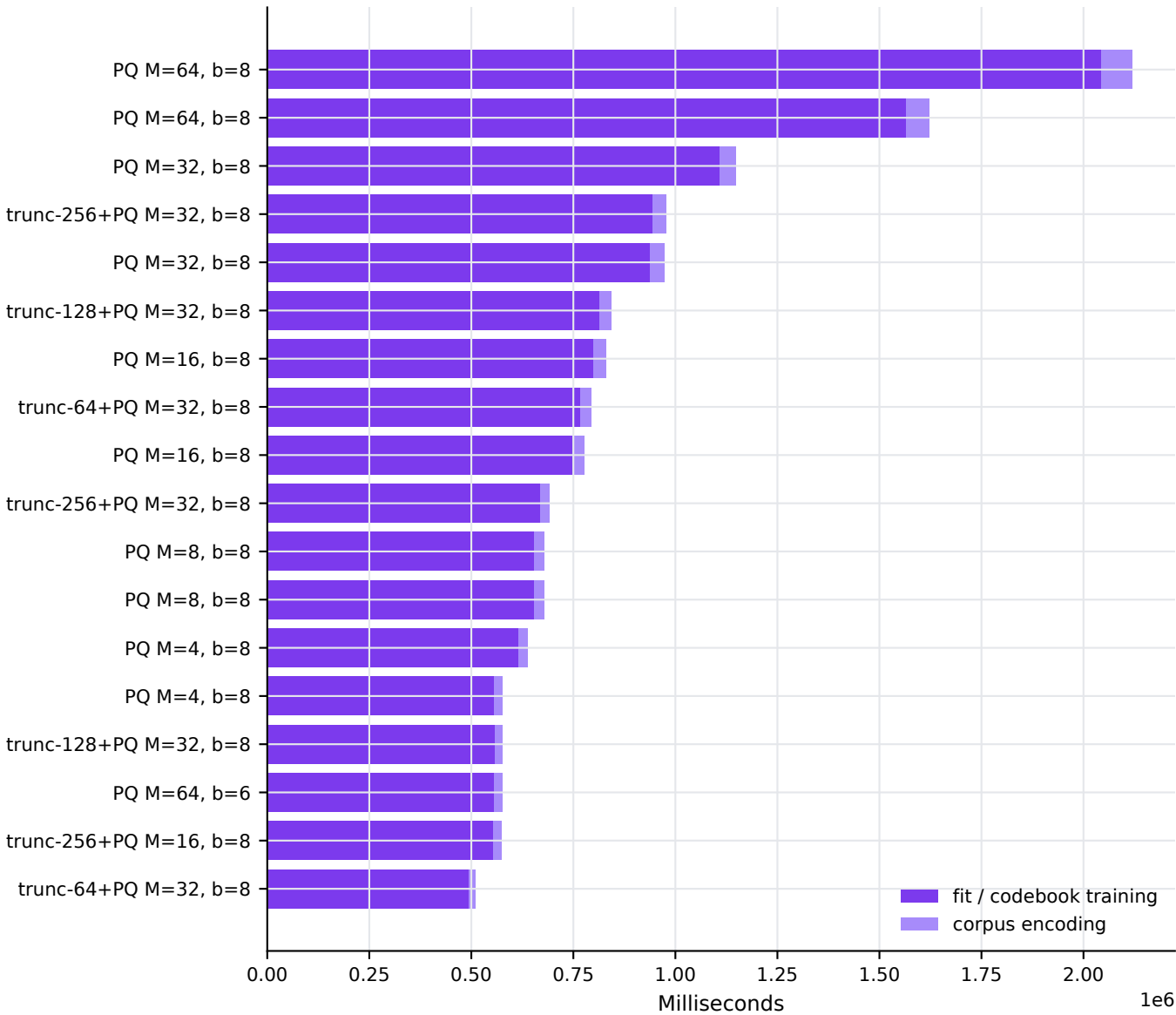
Offline compression cost
