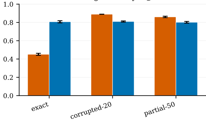
Routing accuracy R@1
