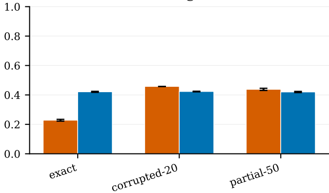
nDCG@10
