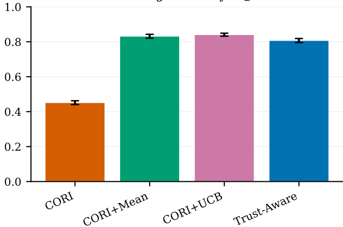
Routing accuracy R@1
