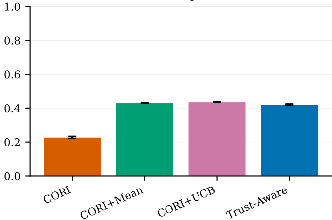
nDCG@10
