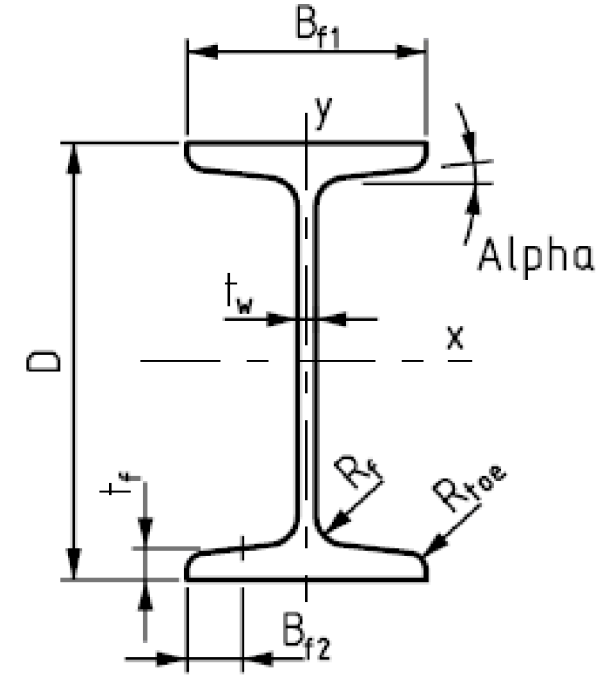
S SECTION
