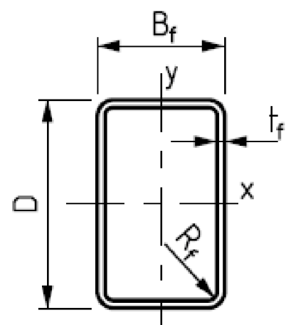
HSS SECTION
