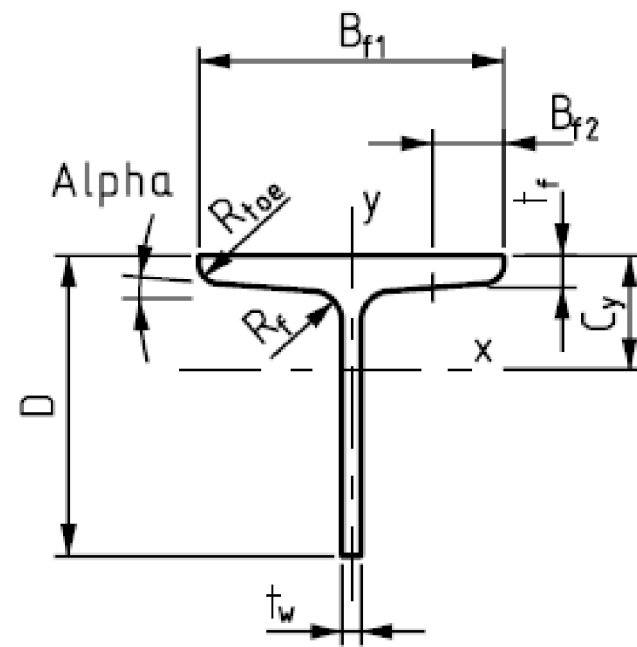
ST SECTION
