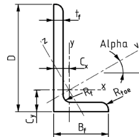
L SECTION
