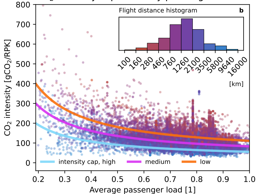
CO 2 intensity cap model by passenger load a
