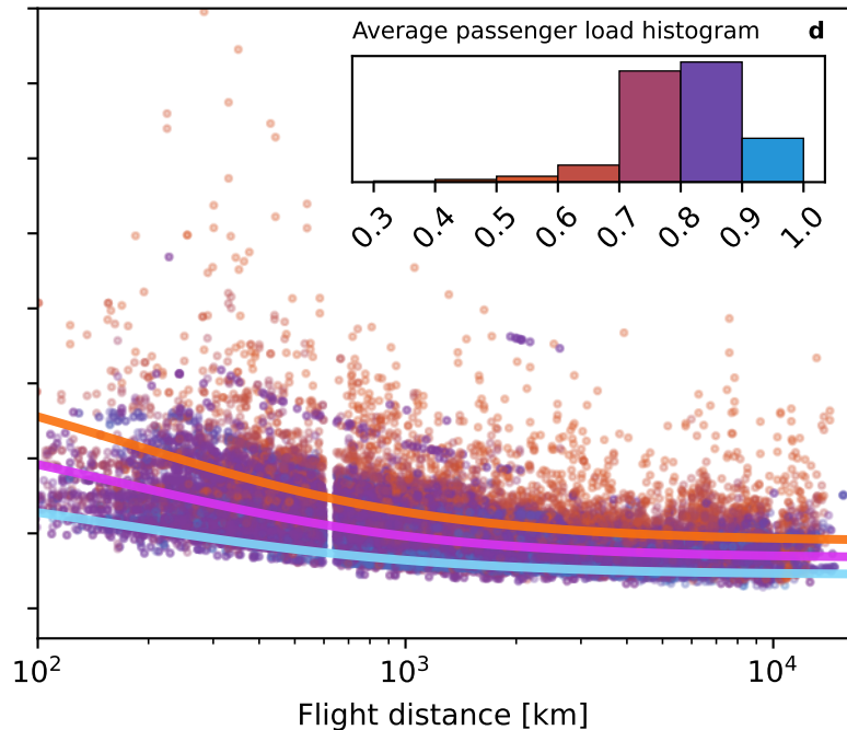
CO 2 intensity cap model by flight distance c
