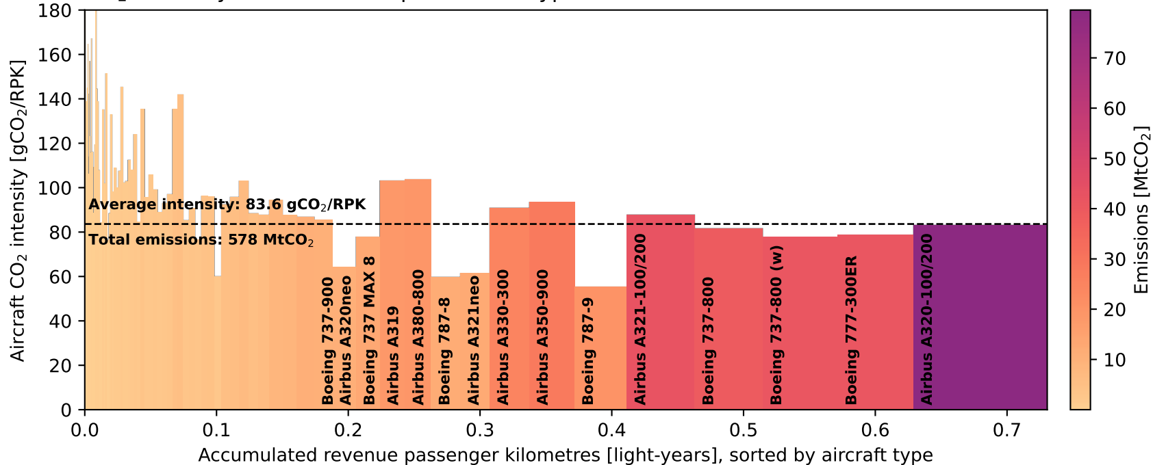
CO 2 intensity and emissions per aircraft type
