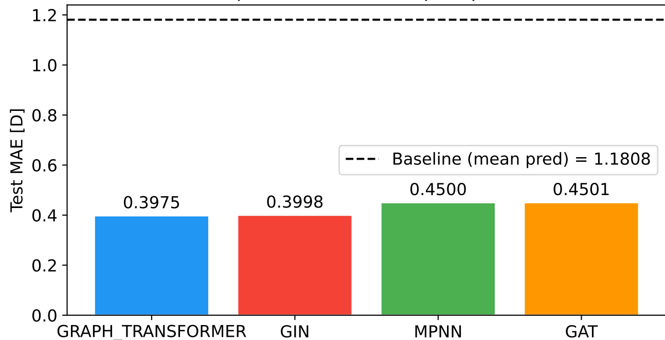
Model Comparison on QM9 — \mu (Dipole Moment)
