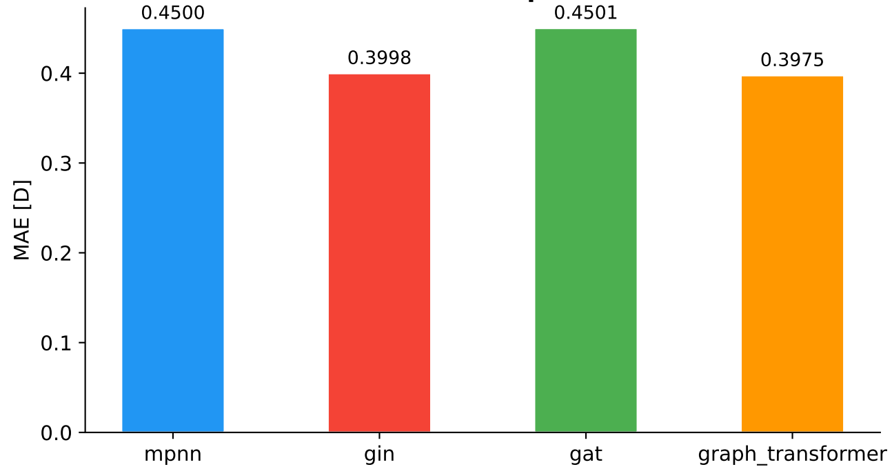
Test MAE Comparison
