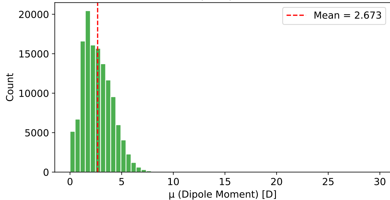
Distribution of \mu (Dipole Moment) [D]
