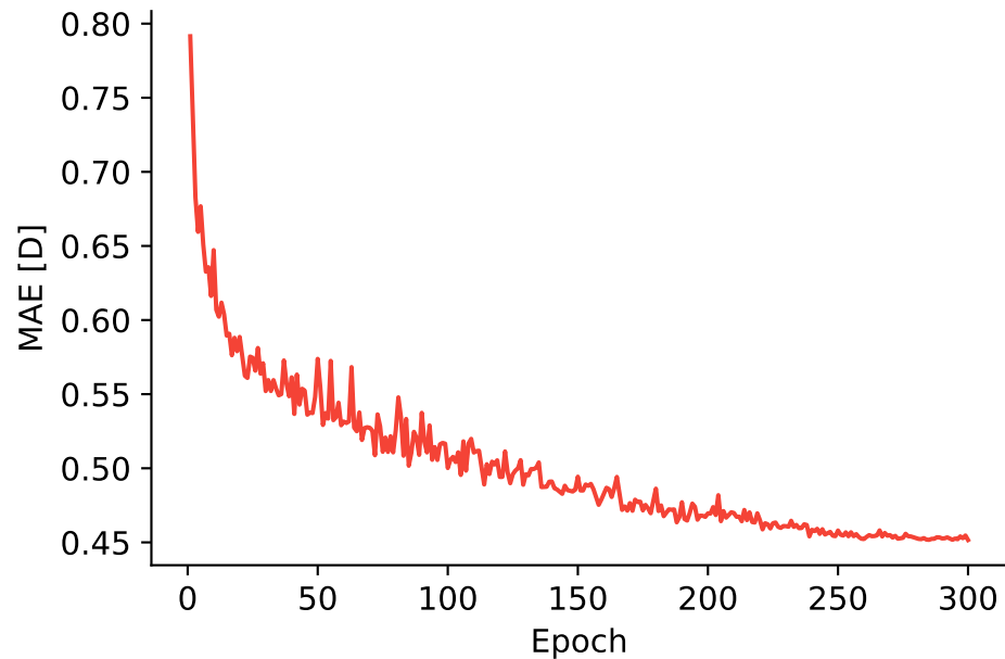
Validation MAE [D]
