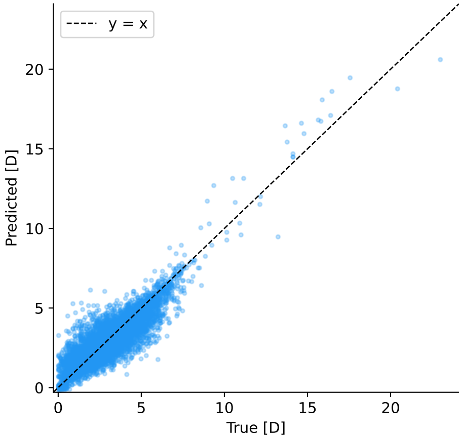
Predictions vs. Ground Truth — gat_seed42
