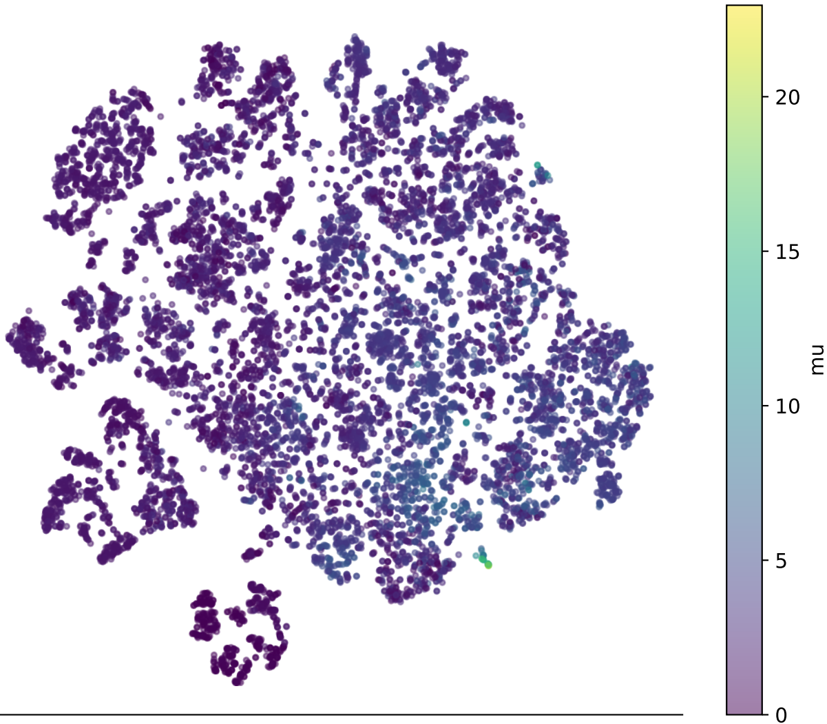
t-SNE of Learned Embeddings — gat_seed42
