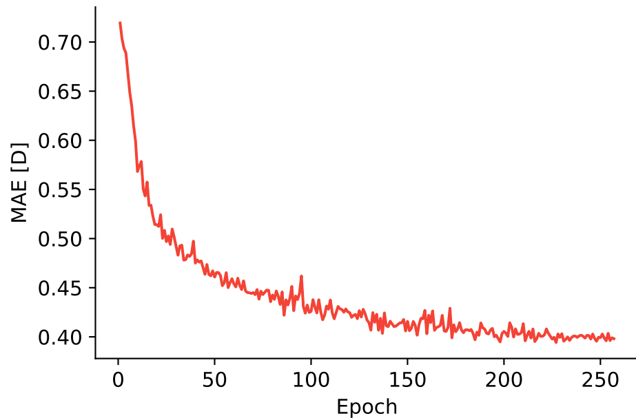
Validation MAE [D]
