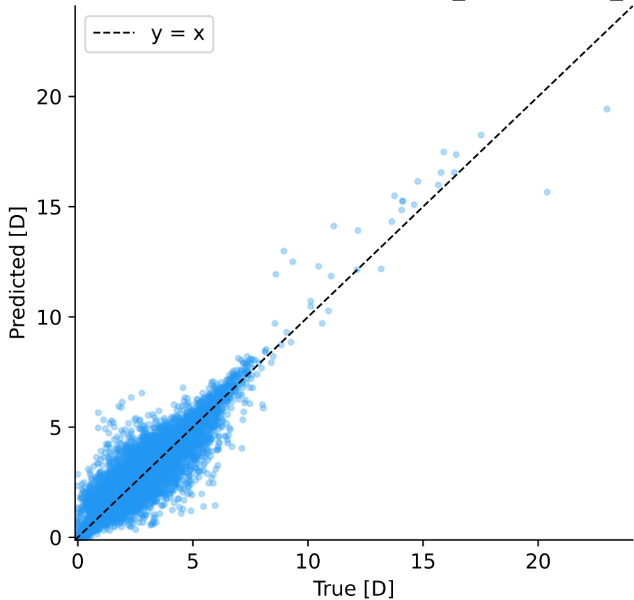
Predictions vs. Ground Truth — graph_transformer_seed42
