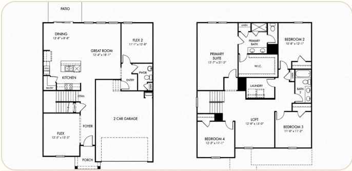
Builder floor plan reference
