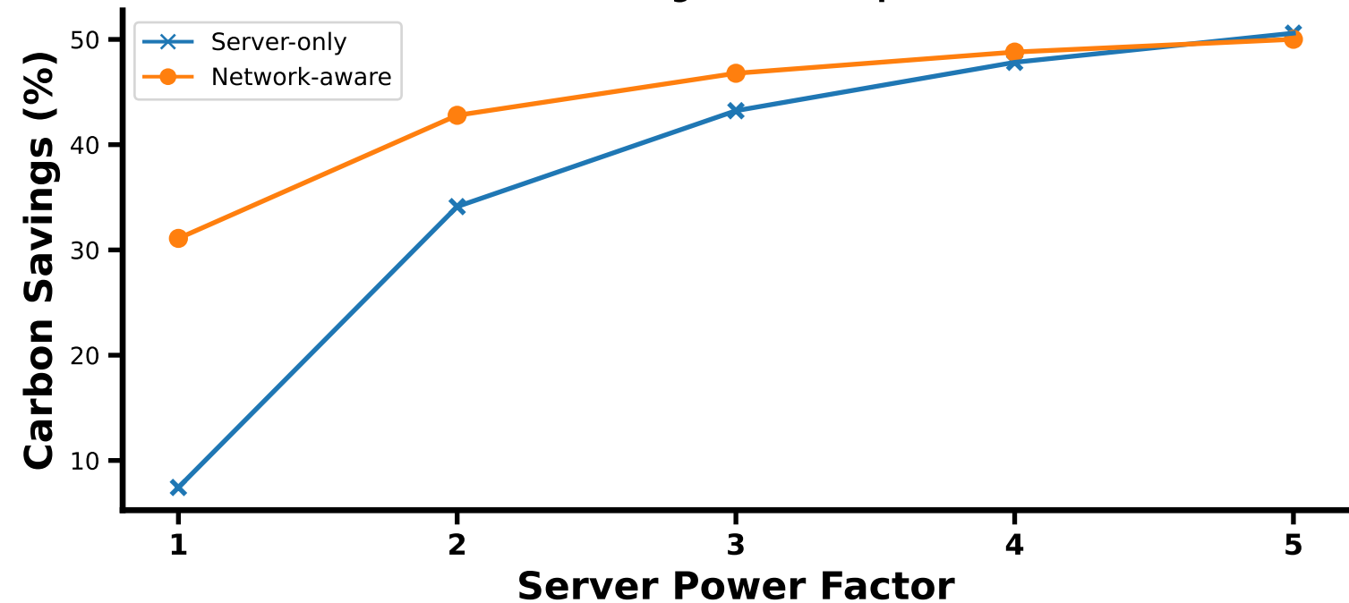
USA carbon savings vs server power factor
