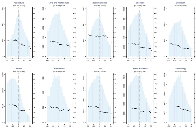
RDD: Retakes PSU Within Two Years by Field Outcome: retakes_psu_2y. Regression BW = \pm 25 ; plot range = \pm 50
