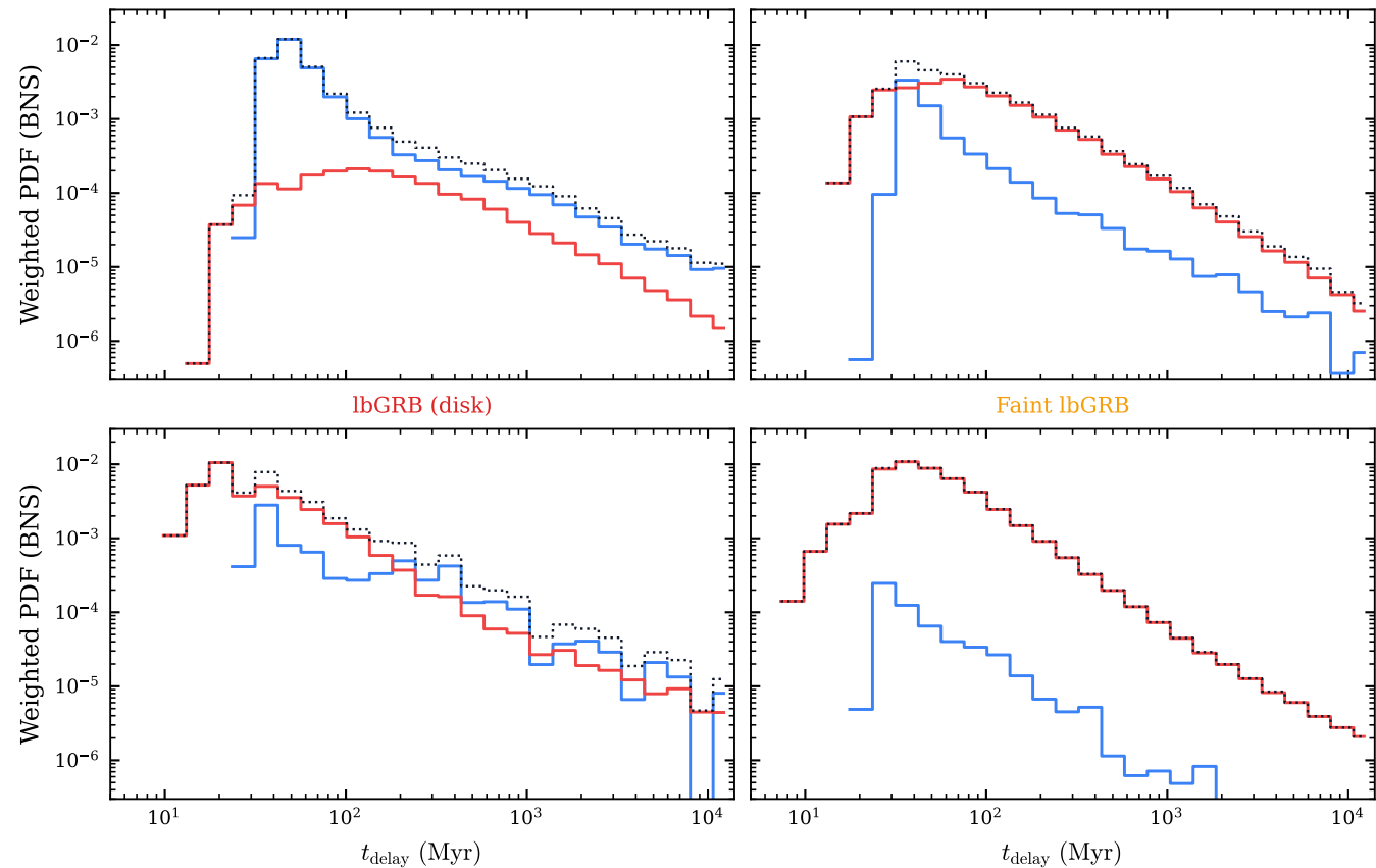
Formation channel
