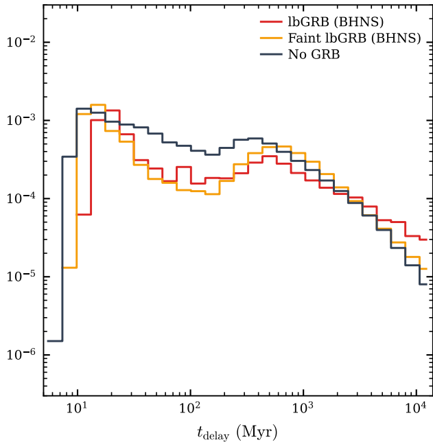
Weighted PDF (BHNS)
