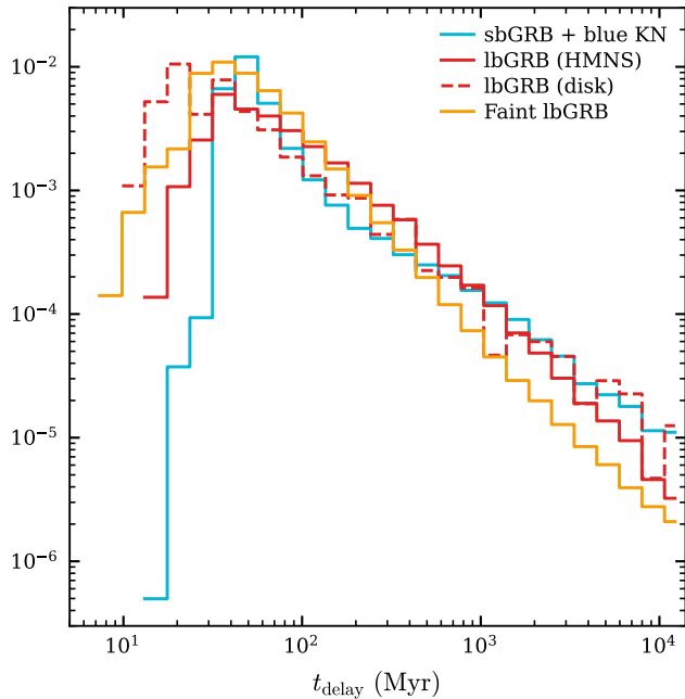
Weighted PDF (BNS)
