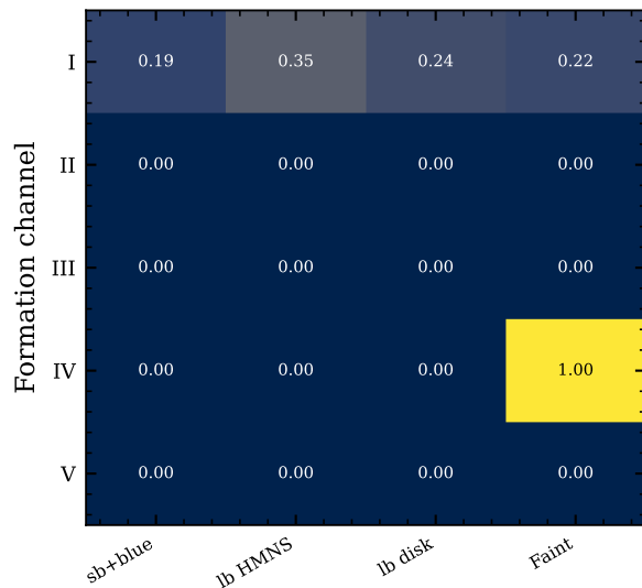
K (optimistic CE)
