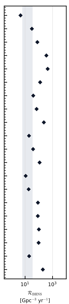
\blacklozenge \mathcal{R}(z=0) LVK NSBH 90% CR
