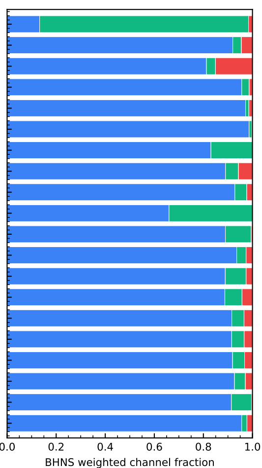
Formation channel I Stable MT + CE II Stable MT only IV Double-core CE
