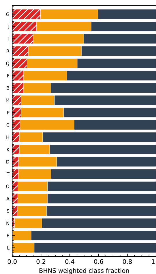
GRB class IbGRB + red KN (BHNS disk) Faint IbGRB (BHNS) No GRB
