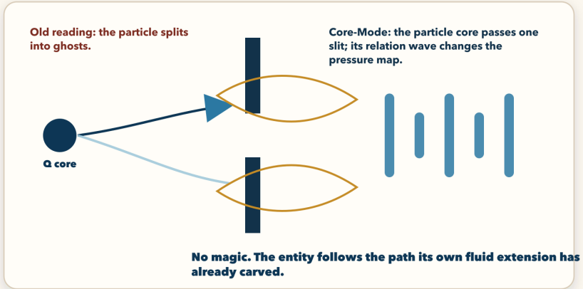
Figure 21: Quantum ghosts as fluid projection
