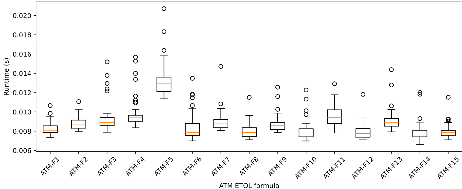
ATM repeated runs: runtime distribution
