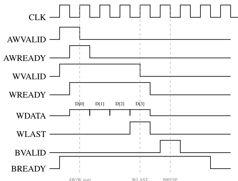
Figure 4.9: AXI4 Cache Write-Back: 4-Beat INCR Write Burst (AWLEN=3)
