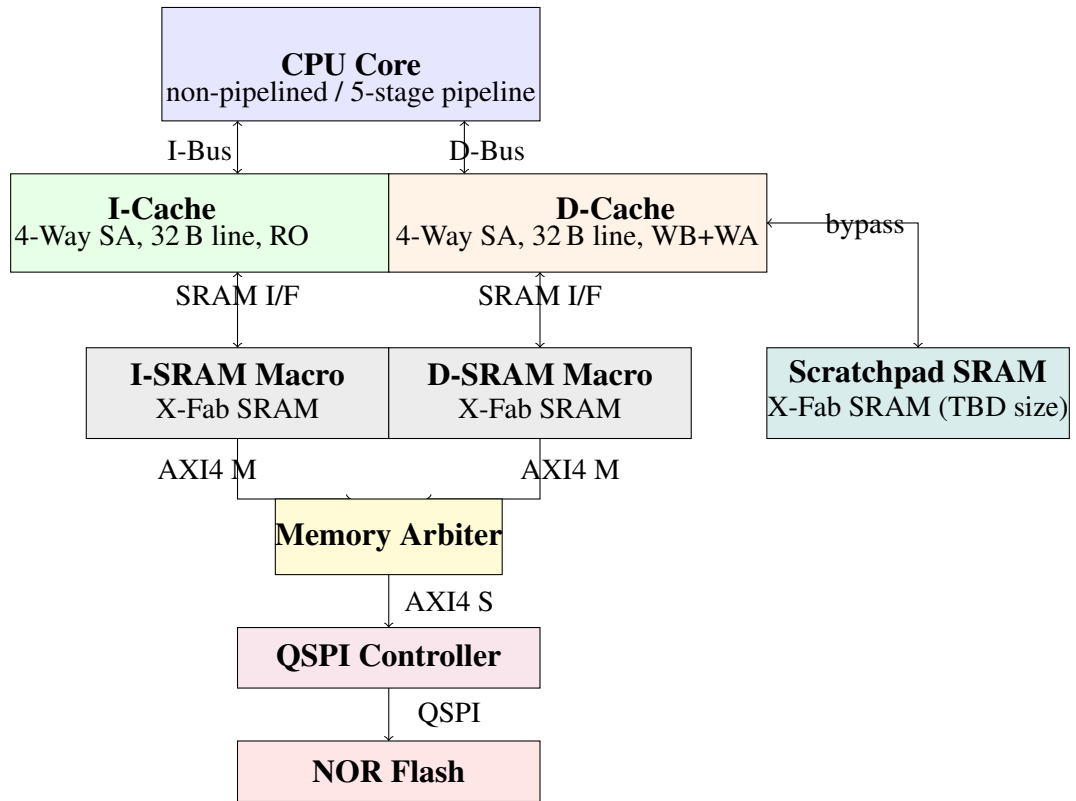
Figure 4.5: System Memory Architecture Block Diagram
