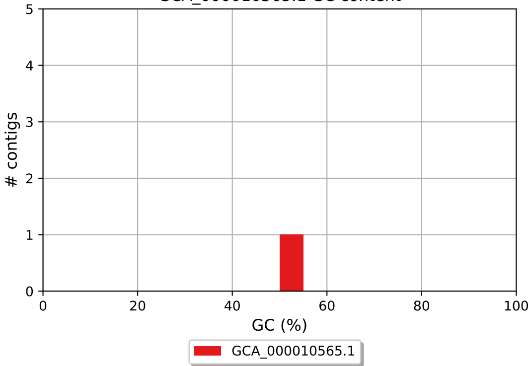
GCA_000010565.1 GC content
