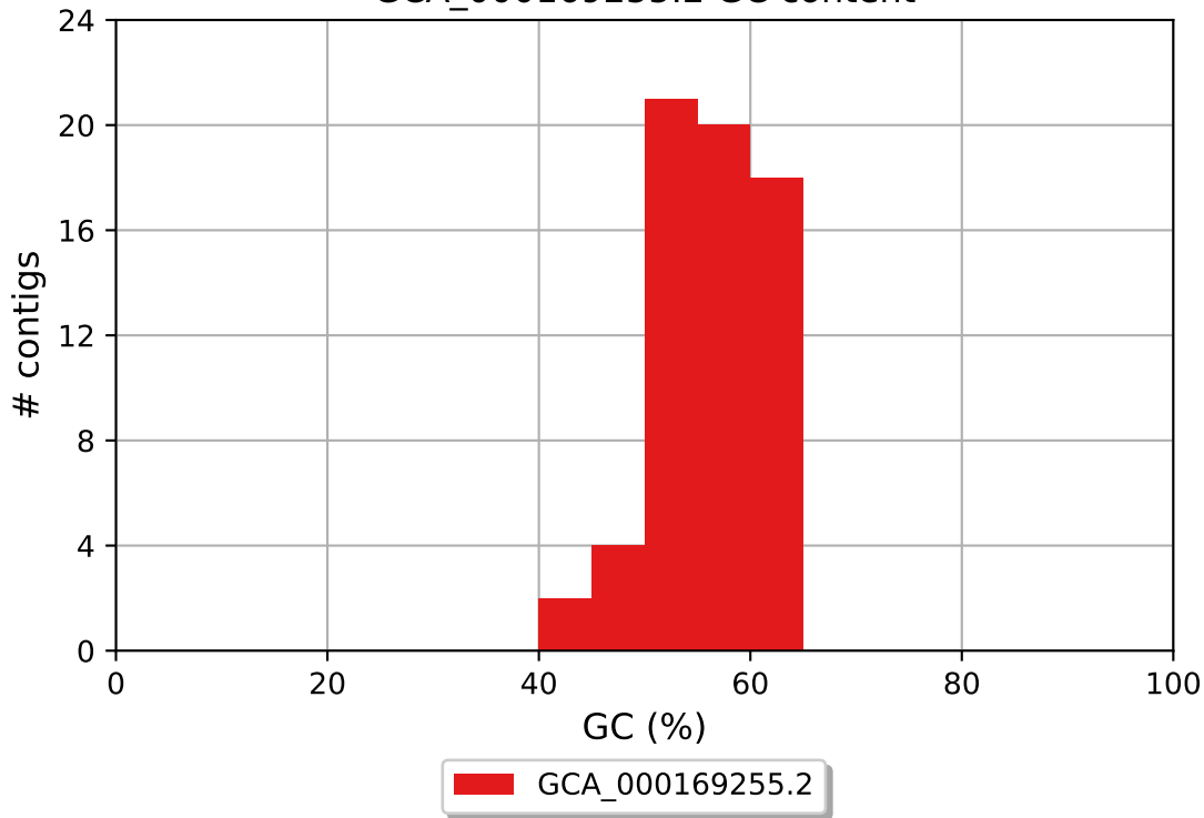
GCA_000169255.2 GC content
