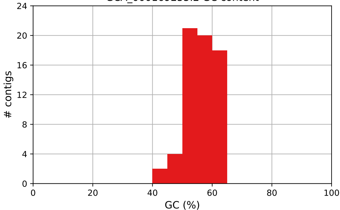
GCA_000169255.2 GC content
