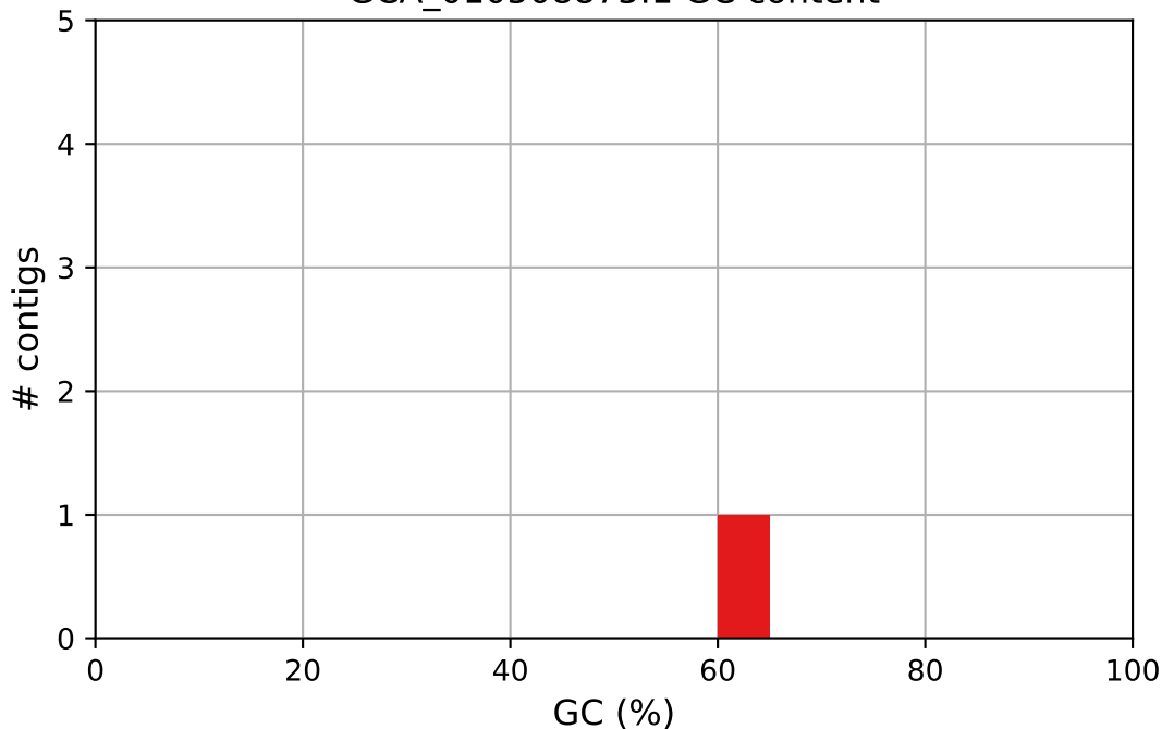
GCA_010508875.1 GC content
