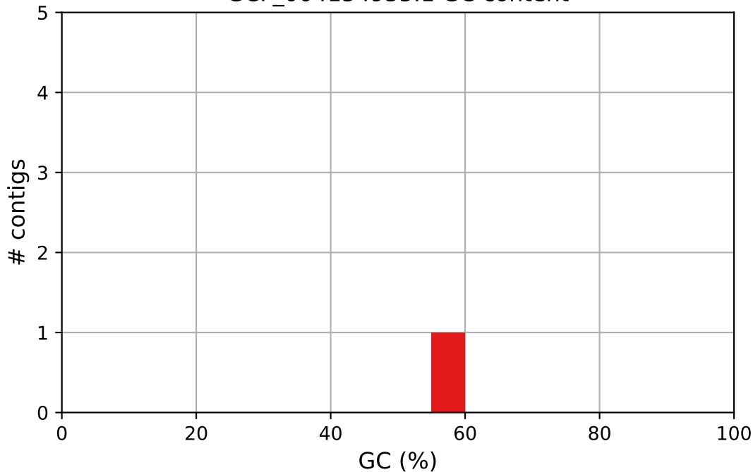
GCF_004154955.1 GC content
