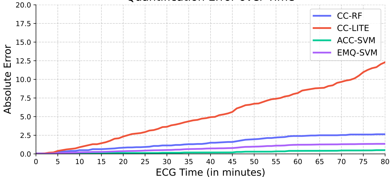
Quantification Error over Time
