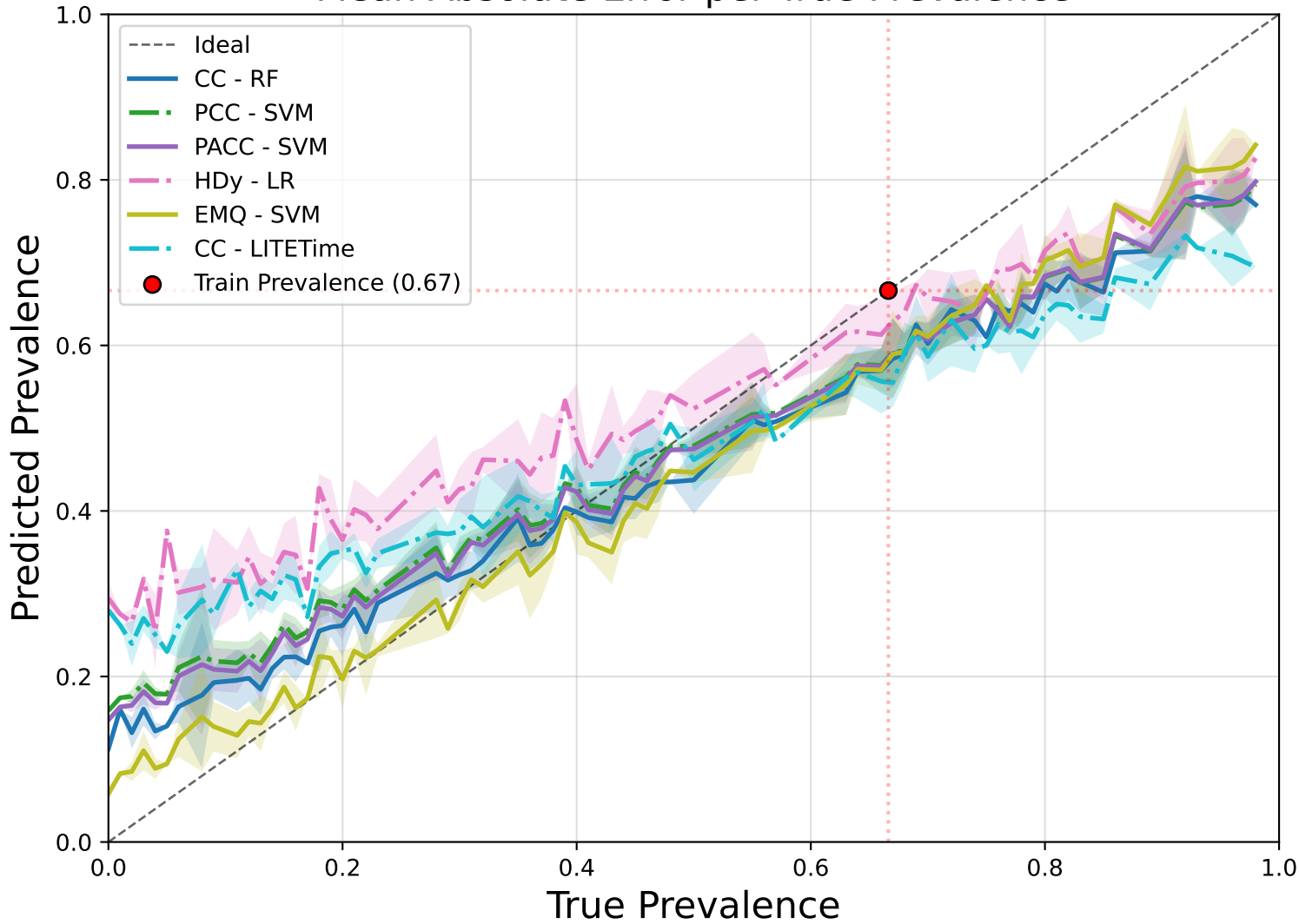
Mean Absolute Error per True Prevalence
