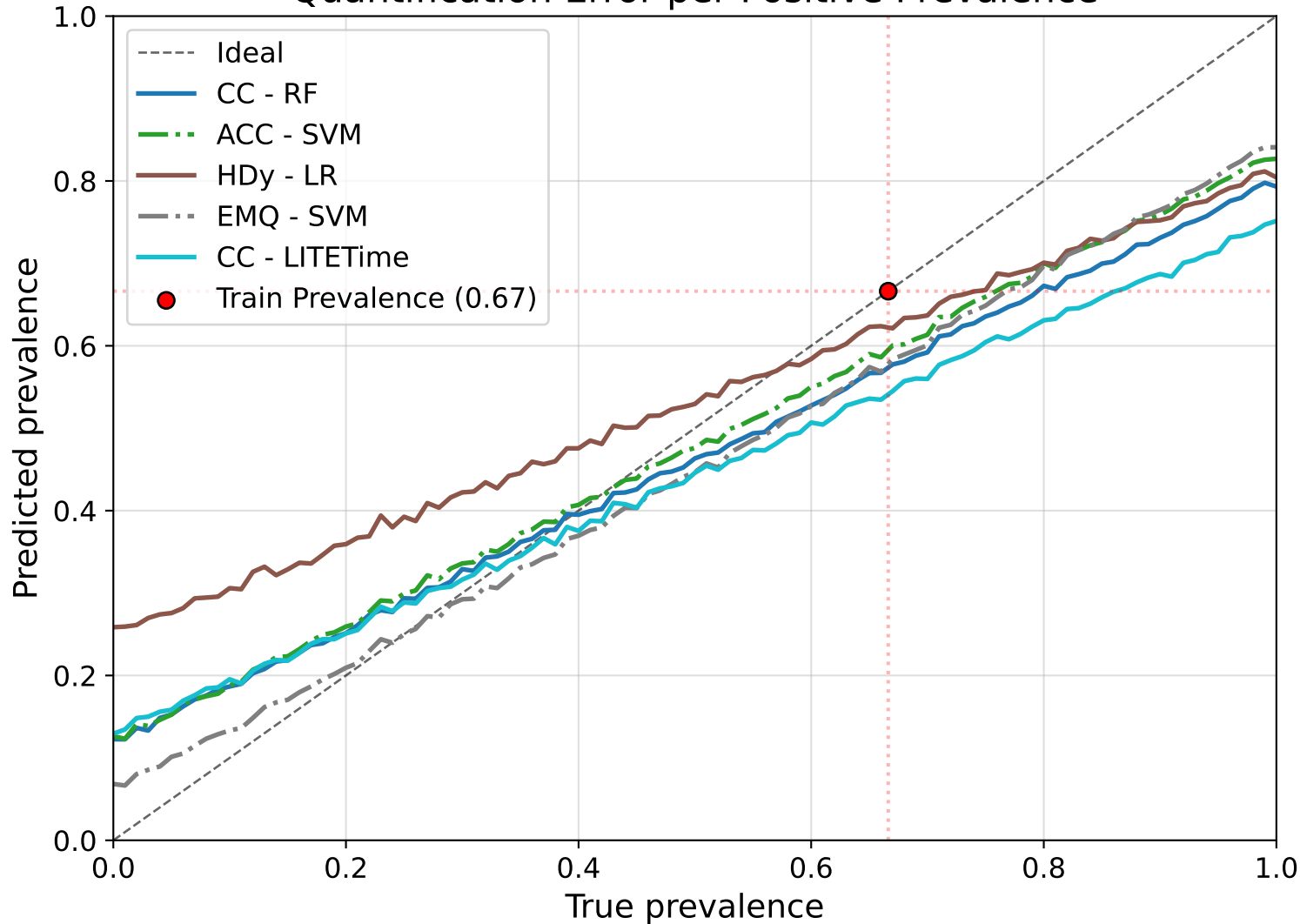
Quantification Error per Positive Prevalence
