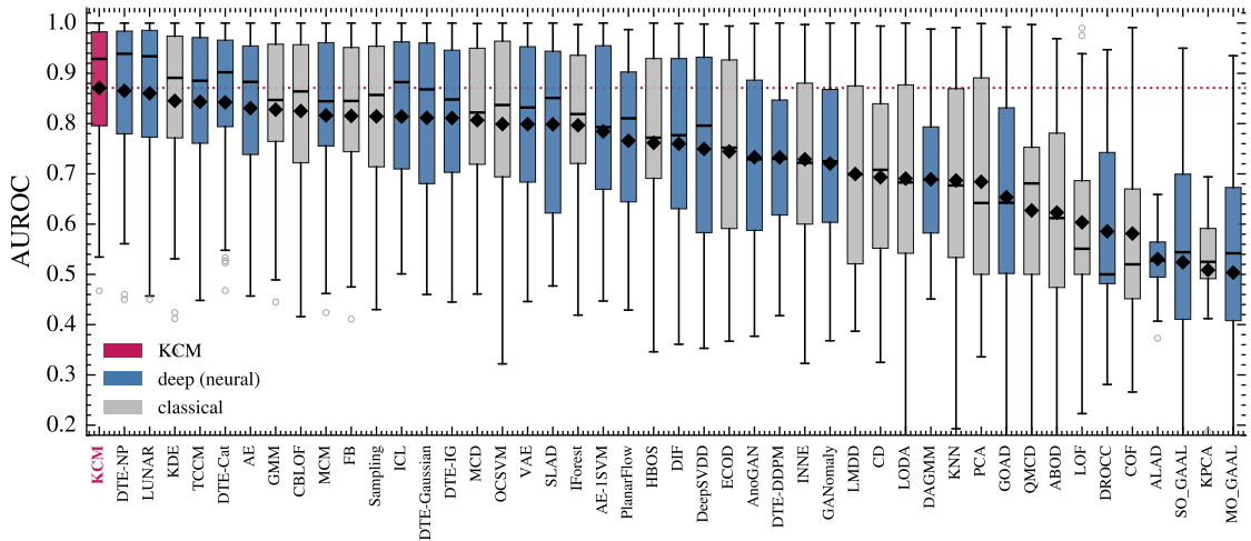
Per-dataset AUROC across the 47 ADBench datasets (methods ordered by mean AUROC; diamond = mean)
