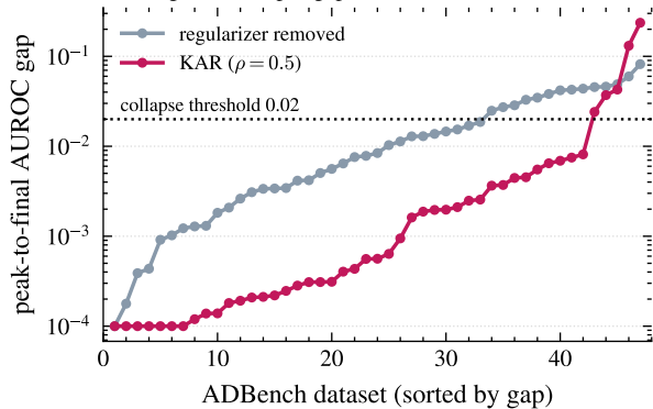
Convergence-collapse gap across the 47 ADBench datasets
