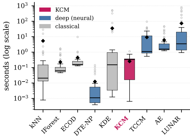
Fit / training time
