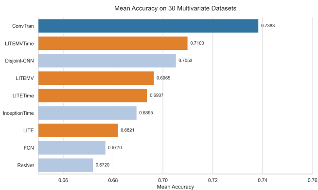
Fig. 7: Mean accuracy comparison on the 30 multivariate datasets. Although LITE-based methods perform competitively, ConvTran holds the leading accuracy.
