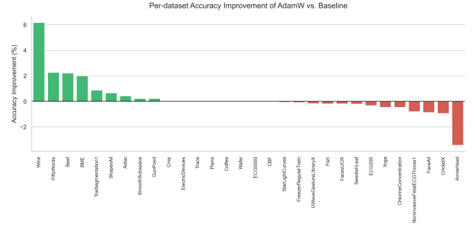
Fig. 4: Per-dataset accuracy improvement of AdamW over baseline.
