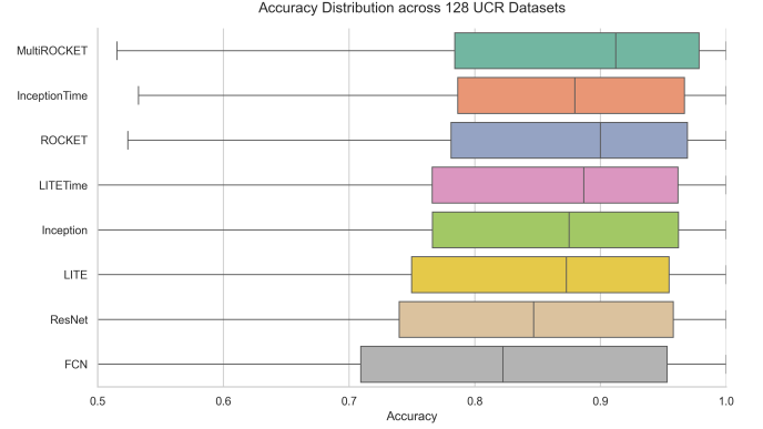
Fig. 2: Performance distribution of LITE and LITETime models against classical and state-of-the-art benchmarks across the 128 UCR datasets.
