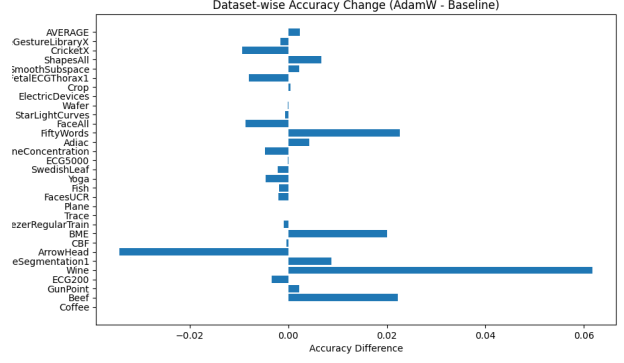
Fig. 4: Per-dataset accuracy improvement of AdamW over baseline.
