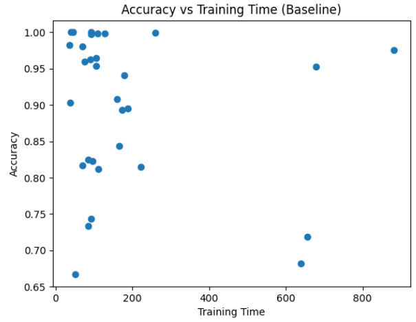
Fig. 5: Accuracy vs. training time trade-off across configurations.
