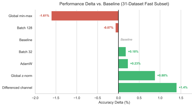
Fig. 3: Performance delta versus baseline (fast subset) across improvement configurations, showcasing the significant gain from the differenced channel.
