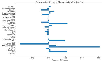
Fig. 4: Per-dataset accuracy improvement of AdamW over baseline.
