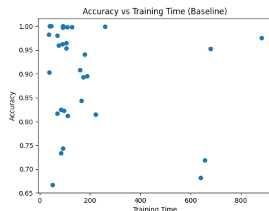
Fig. 5: Accuracy vs. training time trade-off across configurations.
