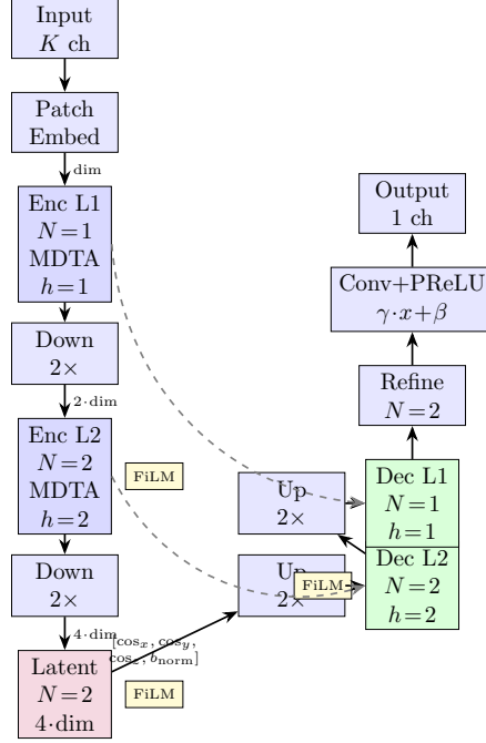
Figure 3: Restormer3D internal architecture for Hybrid RGS. A 3-level encoder-decoder with transformer blocks at each stage. The encoder progressively downsamples spatial dimensions ( \times 2 per level) while doubling channel count ( \text{dim} \rightarrow 2 \cdot \text{dim} \rightarrow 4 \cdot \text{dim} , with \text{dim} = 12 ). Each level contains N transformer blocks combining Multi-DConv Head Transposed Self-Attention (MDTA, h heads) and Gated-DConv Feed-Forward Networks (GDFN). The decoder mirrors the encoder with skip connections (dashed gray arrows) and channel-reduction convolutions after concatenation. Refinement blocks and a learned affine output head ( \gamma_{\text{out}}x + \beta_{\text{out}} ) produce the single-channel denoised volume. Optional FiLM conditioning (yellow boxes) modulates features at three stages using the target gradient’s acquisition metadata [\cos_x, \cos_y, \cos_z, b_{\text{norm}}] ; see Table 6 for evaluation. The 2D counterpart, Restormer-2D, shares this same topology (Figure 4) but with 2D Conv2d /MDTA/GDFN operations and PixelUnshuffle / PixelShuffle resampling in place of Conv3d /volumetric MDTA and strided Conv3d / ConvTranspose3d .
