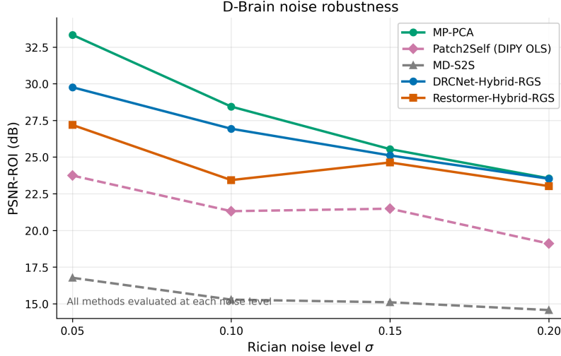
Figure 6: Noise-robustness curve on D-Brain. The plot shows PSNR-ROI versus Rician noise level \sigma \in \{0.05, 0.10, 0.15, 0.20\} for MP-PCA, Patch2Self, MD-S2S, DRCNet-Hybrid-RGS, and Restormer-Hybrid-RGS, with missing baseline points omitted where runs are unavailable.
